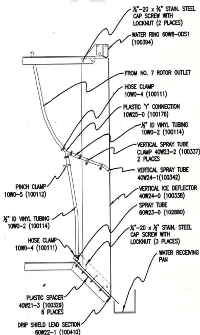
DETAIL 1 - VERTICAL ICE DEFLECTOR
